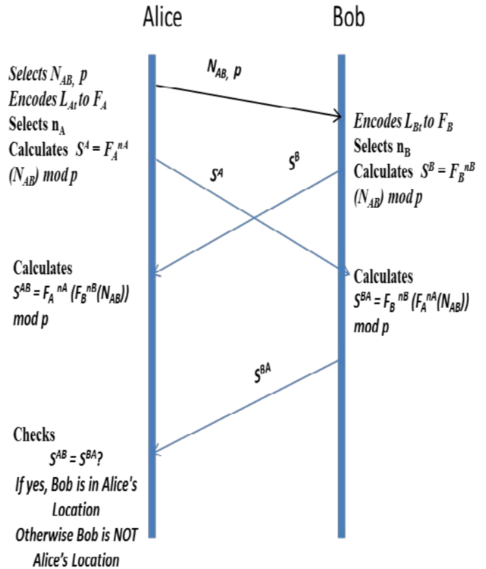
Fig 2. The L4NE Protocol
