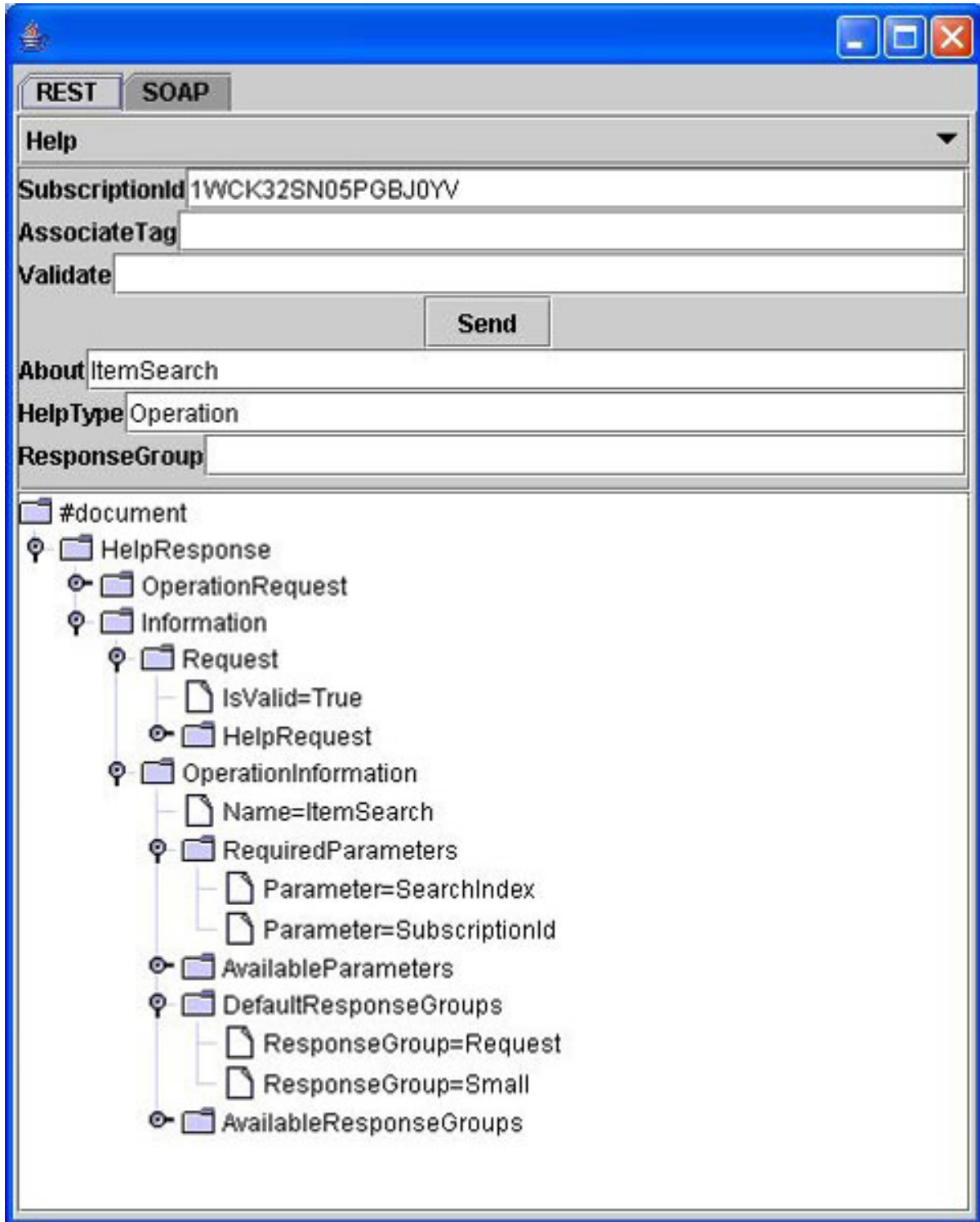
Figure 4. The Help operation
