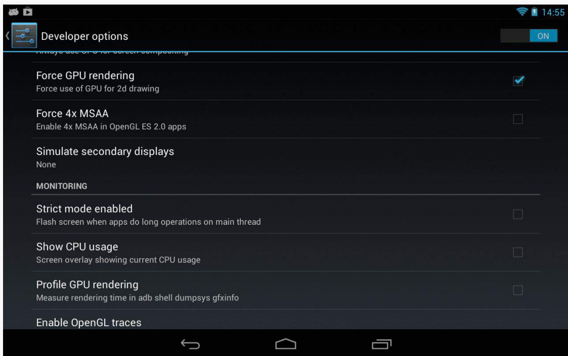
Figure 645: Developer Options, Showing “Force GPU rendering” and “Profile GPU rendering”
