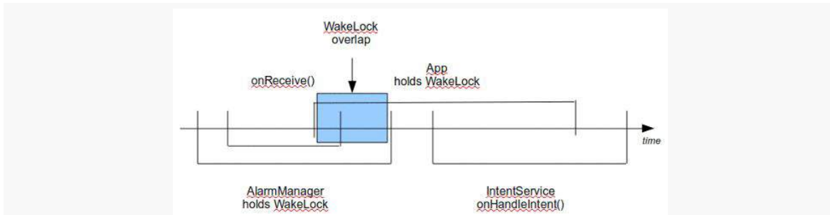
Figure 569: The WakeLock Overlap
