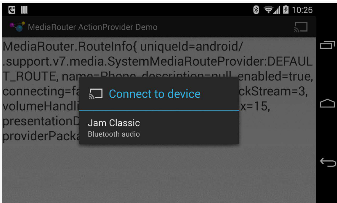
Figure 519: MediaRouter ActionProvider Demo, on a Nexus 4, Showing Available Routes
