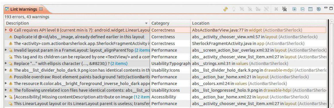
Figure 623: Eclipse Lint Warnings View
