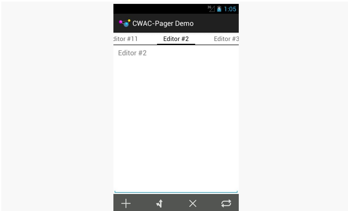
Figure 457: ArrayPagerAdapter Demo App, Showing Result of “Add” From Second Page
