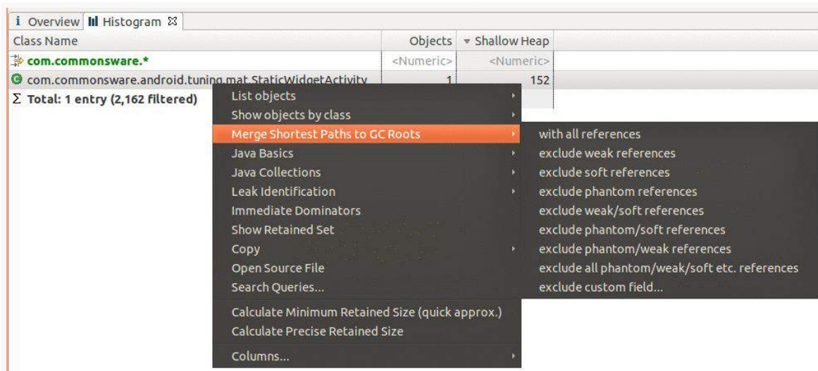
Figure 678: A filtered histogram, showing com.commonware.* objects
