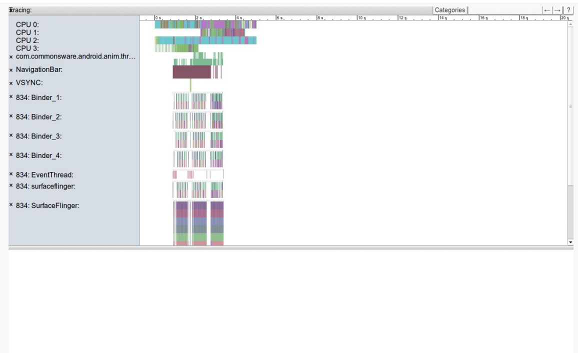
Figure 650: Systrace Output, As Initially Viewed
