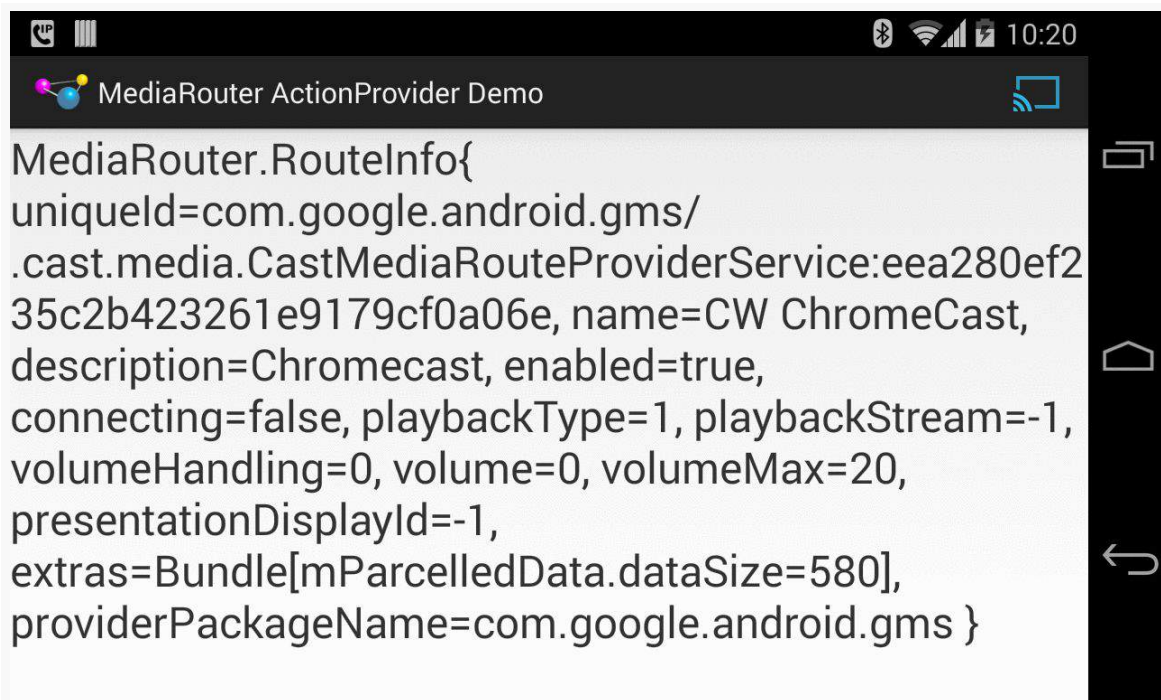
Figure 524: MediaRouter ActionProvider Demo, on a Nexus 4, Showing Selected Chromecast Route
