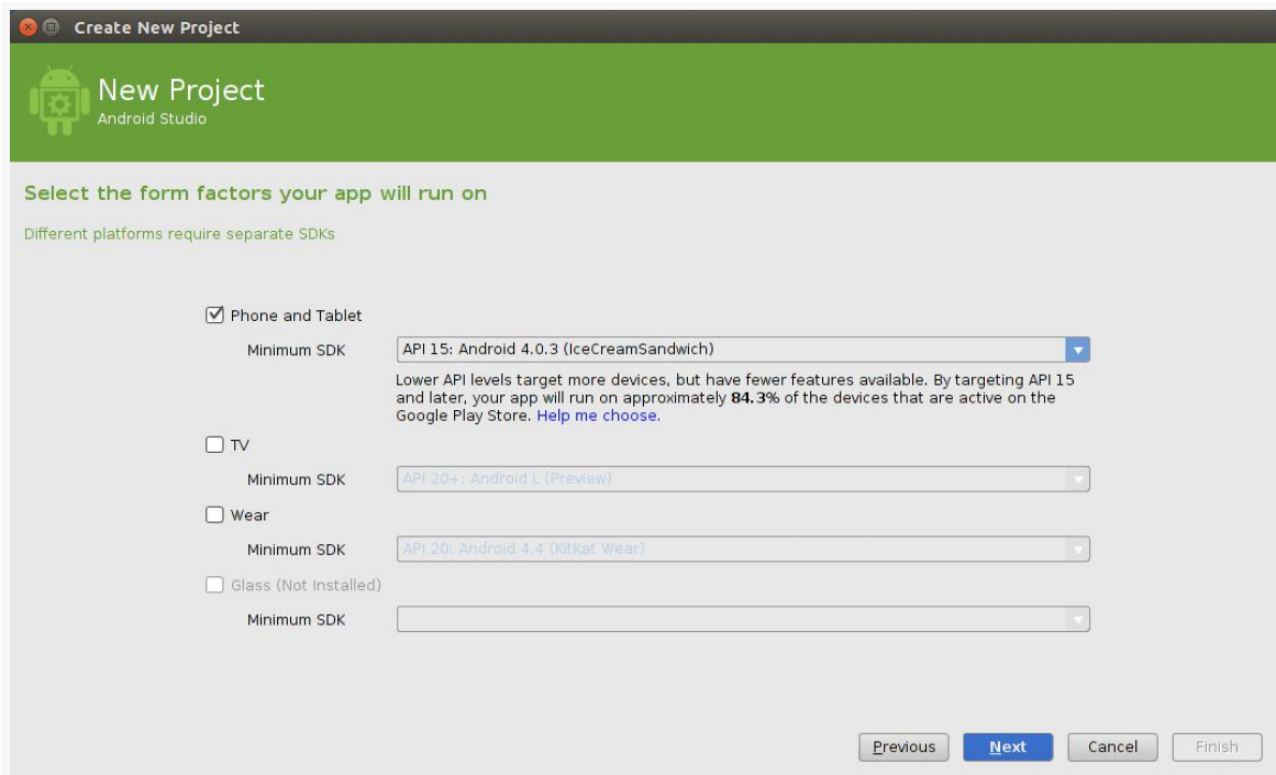
Figure 12: Android Studio Create-Project Wizard, Second Page
