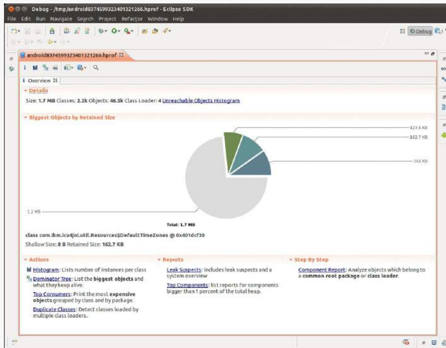
Figure 674: The Overview tool inside the MAT Eclipse perspective
