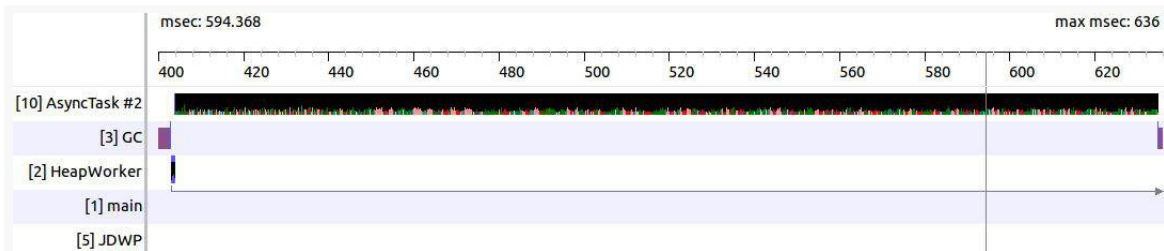
Figure 643: Traceview, zoomed in on ~230 milliseconds of run time
