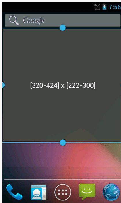
Figure 482: Resize Widget, During Resize Operation
