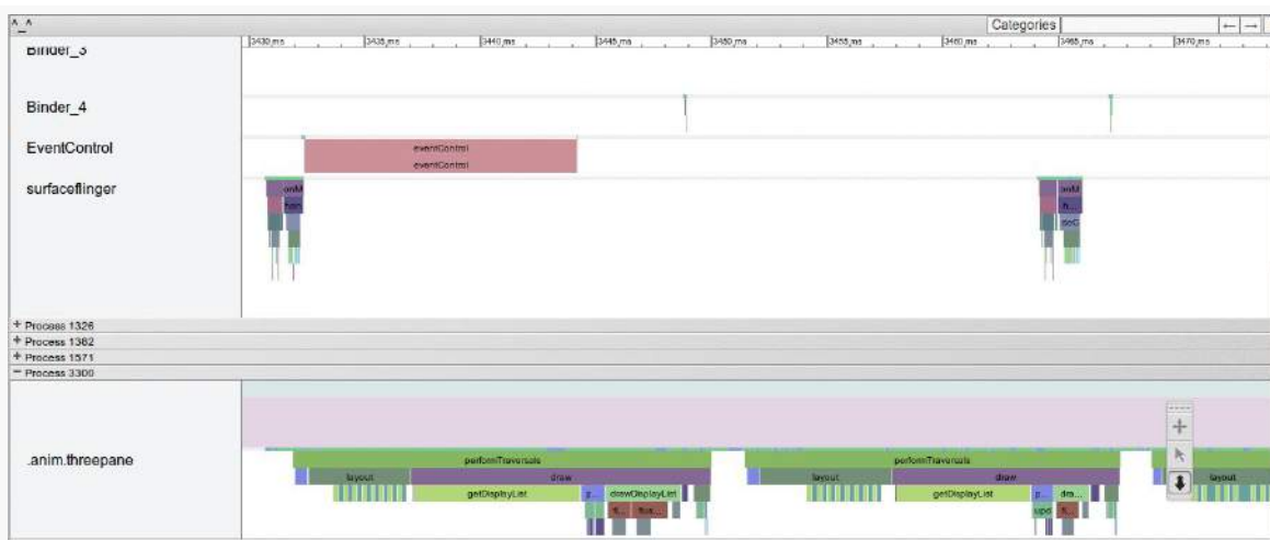
Figure 652: Systrace Output, Zoomed In on 40 Milliseconds of Profiling
