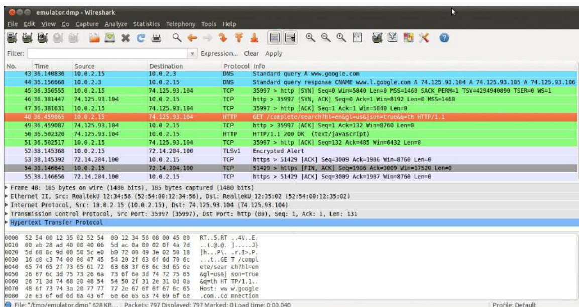
Figure 665: Wireshark examining captured emulator packets
