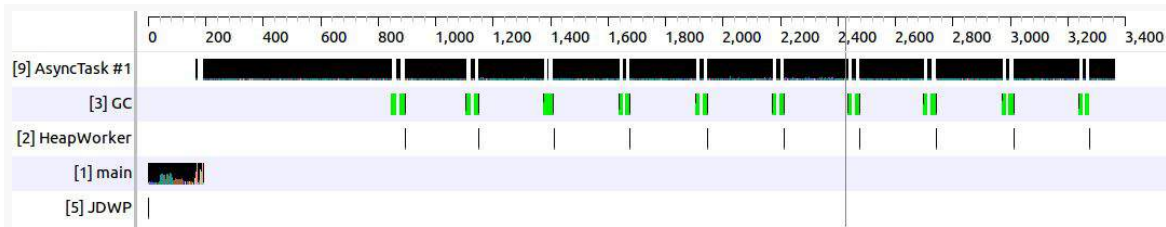
Figure 638: Zoomed in look at the TraceView thread timelines
