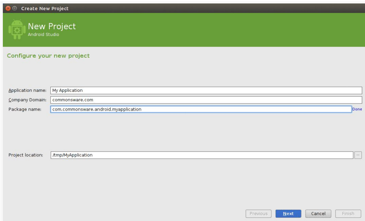
Figure 11: Android Studio Create-Project Wizard, First Page, with Editable Package Name
