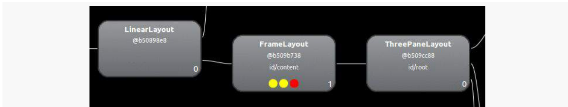
Figure 660: Single-Child FrameLayout in Three-Pane Demo, from Hierarchy View
