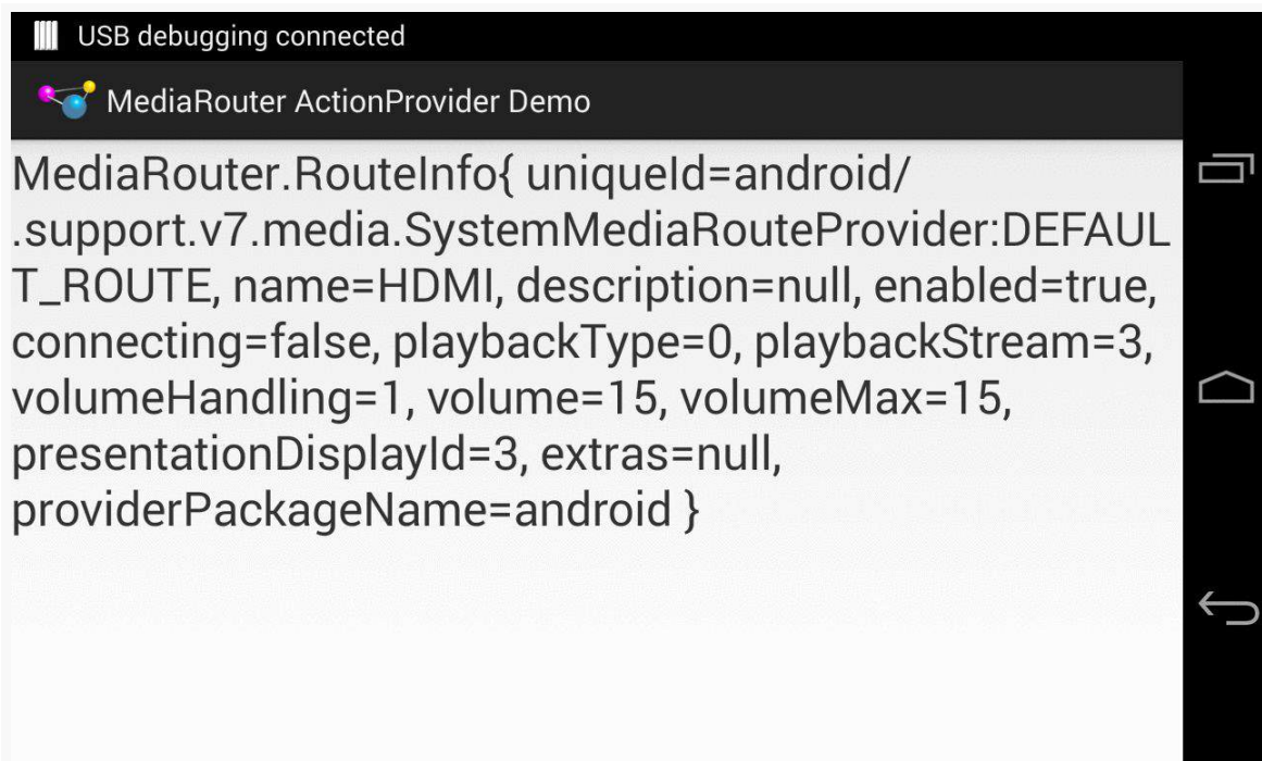
Figure 520: MediaRouter ActionProvider Demo, on a Nexus 4, Showing Live Video Route
