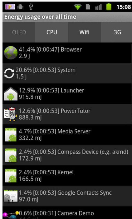
Figure 695: The PowerTutor application roster
